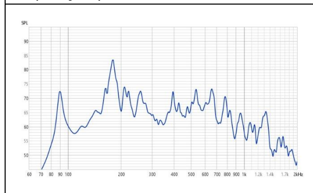
Frequency response
